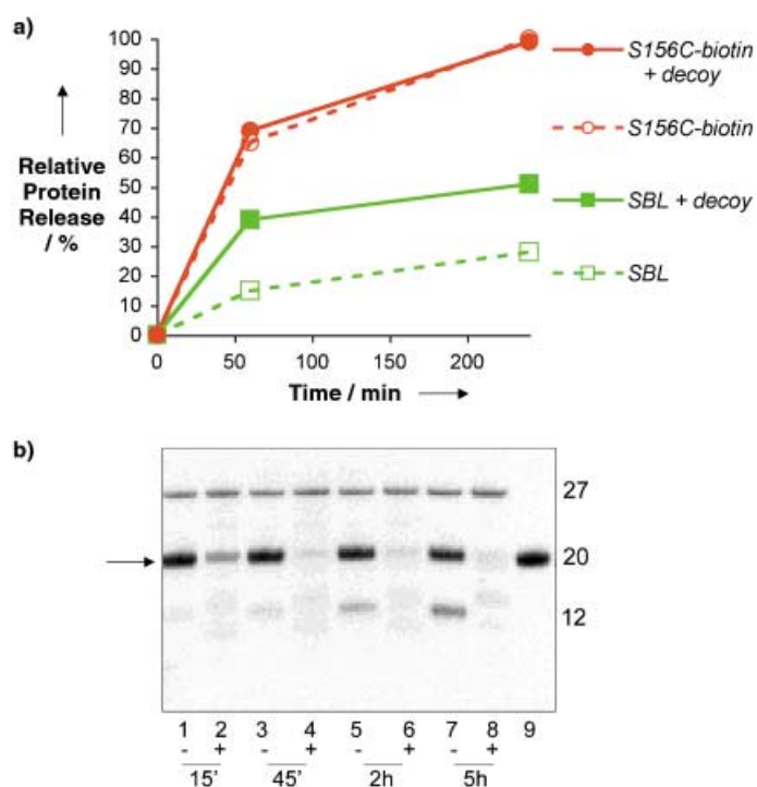
Figure 2. Targeted avidin destruction as measured by (a) peptide production and (b) SDS PAGE. a) The degradation of avidin by targeted S156C-biotin (red) or untargeted WT SBL (green) as determined by the creation of protein fragments ( < 3000 \text{ MW} ) as a function of time in the absence (open symbols and dashed lines) or presence (closed symbols and solid lines) of decoy protein (disulfide scrambled RNase-A). b) Degradation of avidin in the presence of untargeted SBL or S156C-biotin as a function of time. After incubation for 15 min, 45 min, 2 h, and 5 h, samples were inhibited with phenylmethylsulfonyl fluoride then boiled in the presence of SDS and subjected to SDS-PAGE. The upper band (27 000 MW) is untargeted WT SBL (–) or S156C-biotin (+), while the lower band (20 000 MW) indicated with an arrow is that of the avidin target (Lane 9 = avidin control). Elimination of the avidin band is seen for samples incubated with S156C-biotin and little or no diminution of the avidin band is detected for even the longest incubation with untargeted WT SBL (Lanes 1–8).
