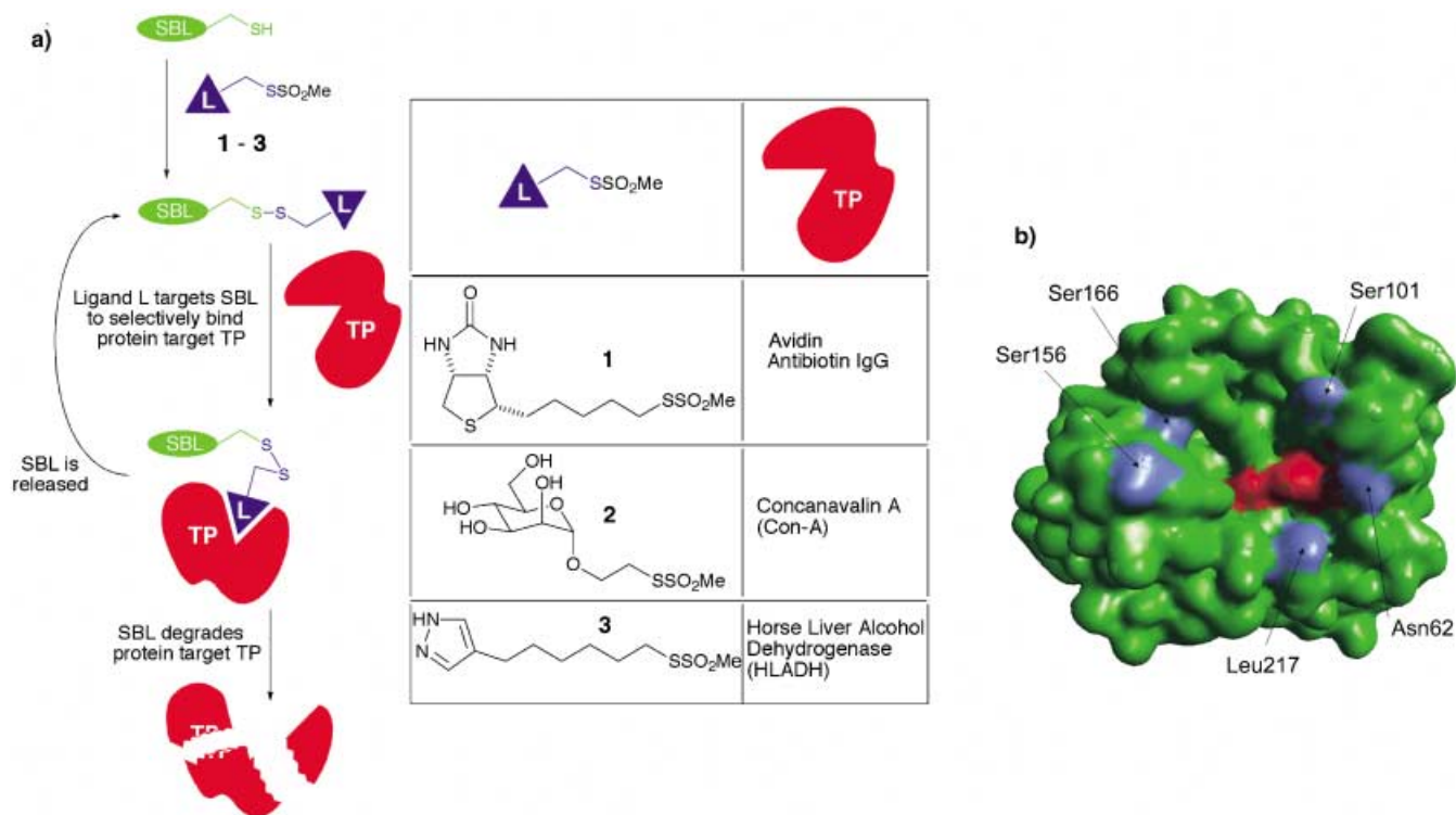
Figure 1. a) The concept of a catalytic antagonist (CA) and its creation. The thiol group of single-point cysteine subtilisin (from Bacillus lentus ; SBL) mutants is chemoselectively modified with targeting ligand (L) by using the appropriate methanethiosulfonate (MTS) reagent (1–3 in this study) to give a CA. For example, L-MTS + S156C subtilisin can be used to create CA S156C-L. The target protein (TP) binds L at its complementary site, thereby juxtaposing the TP and the active site of the SBL chimera. By virtue of this proximity, enhanced CA-catalyzed hydrolytic degradation of TP ensues. The structures of the MTS reagents, which contain natural ligands or inhibitors, used to introduce L and their corresponding TPs are shown in the box; b) The five positions (blue), Asn62, Ser101, Ser156, Ser166, and Leu217 in SBL selected for attachment of targeting ligands. The residues that form the catalytic triad, Asp32, His64, Ser221, are colored red.
