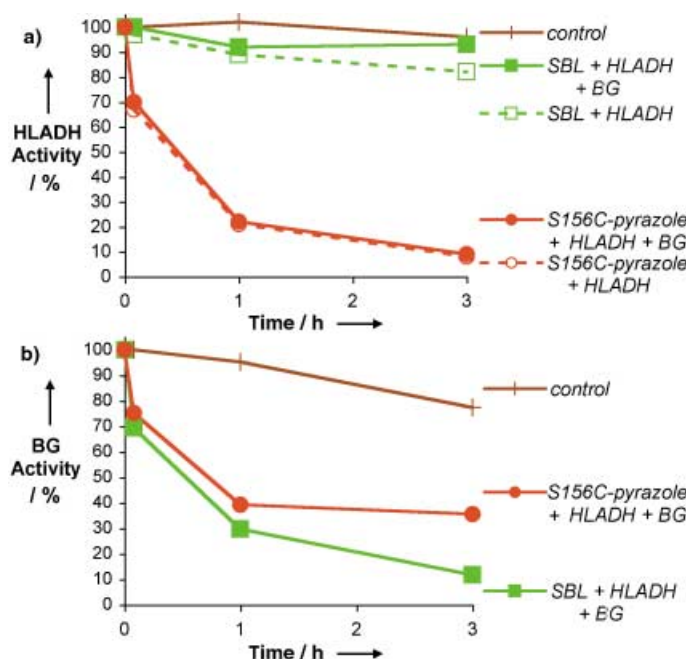
Figure 3. Enhanced destruction of HLADH. a) The degradation of enzymatic activity of HLADH alone (+ HLADH, dashed lines and open symbols) or in a mixture with a second, decoy enzyme BG (+ HLADH + BG, solid lines and closed symbols) by targeted S156C-pyrazole (red) or untargeted WT SBL (green). b) The enzymatic activity of BG in a two-protein mixture of HLADH + BG degraded by targeted S156C-pyrazole (red) or untargeted WT SBL (green).
